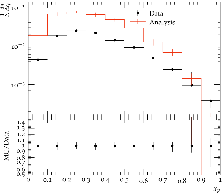
\Lambda^0 Scaled momenta distribution for the Q^2 range 10 to 100 \text{GeV}^2 .
