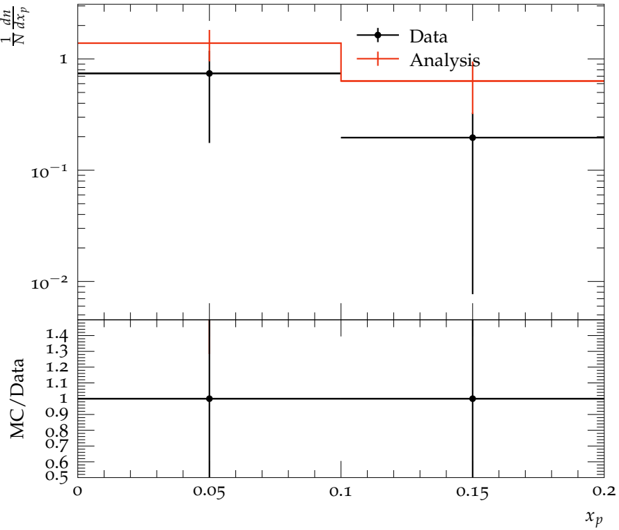
\Lambda^0 Scaled momenta distribution for the Q^2 range 2560 to 10240 GeV
