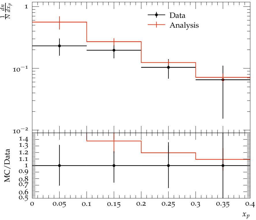
\Lambda^0 Scaled momenta distribution for the Q^2 range 640 to 2560 GeV^2
