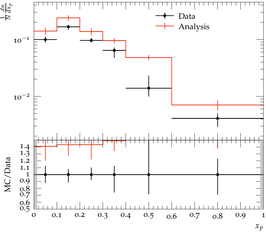
\Lambda^0 Scaled momenta distribution for the Q^2 range 160 to 640 GeV^2 .
