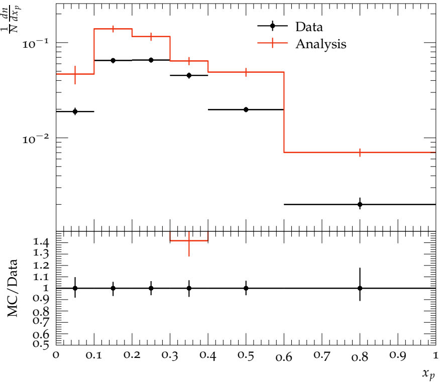
\Lambda^0 Scaled momenta distribution for the Q^2 range 40 to 160 \text{GeV}^2 .
