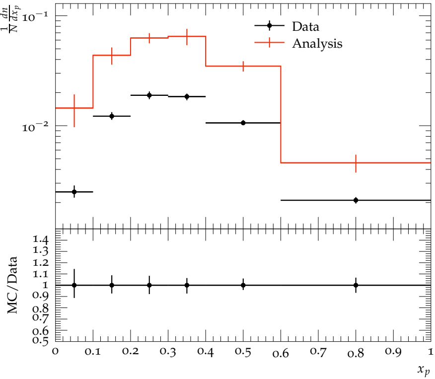
\Lambda^0 Scaled momenta distribution for the Q^2 range 10 to 40 GeV^2 .
