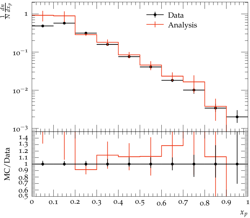
K_S^0 Scaled momenta distribution for the Q^2 range 100 to 1000 GeV^2
