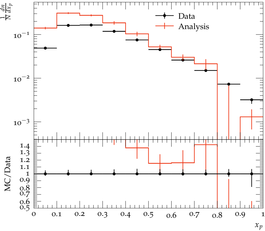
K_S^0 Scaled momenta distribution for the Q^2 range 10 to 100 \text{GeV}^2 .
