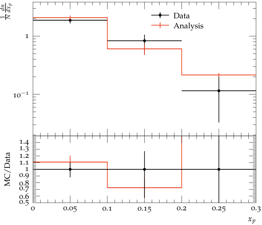
K_S^0 Scaled momenta distribution for the Q^2 range 2560 to 10240 GeV
