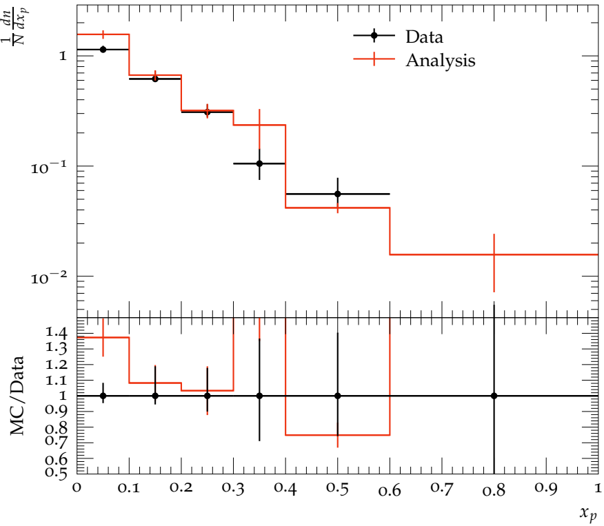
K_S^0 Scaled momenta distribution for the Q^2 range 640 to 2560 \text{GeV}^2
