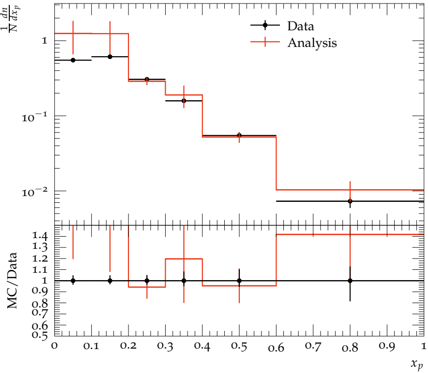
K_S^0 Scaled momenta distribution for the Q^2 range 160 to 640 GeV^2 .
