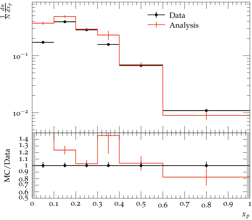
K_S^0 Scaled momenta distribution for the Q^2 range 40 to 160 \text{GeV}^2 .
