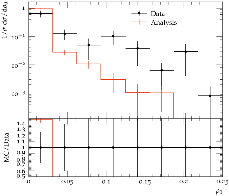
\rho_0 distribution for \langle Q \rangle = 116\text{GeV}
