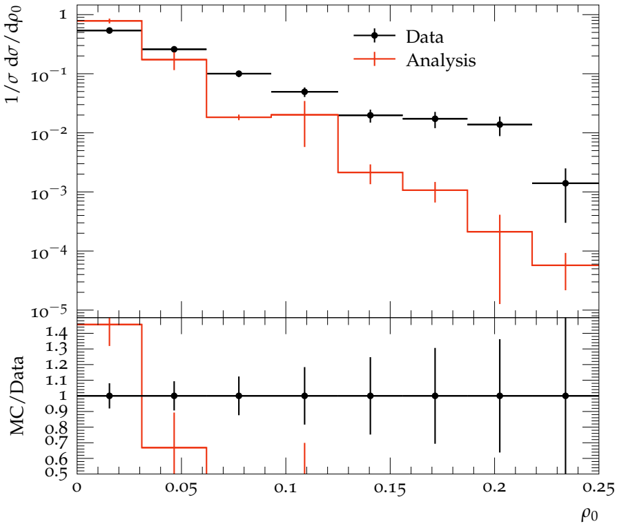
\rho_0 distribution for \langle Q \rangle = 58\text{GeV}
