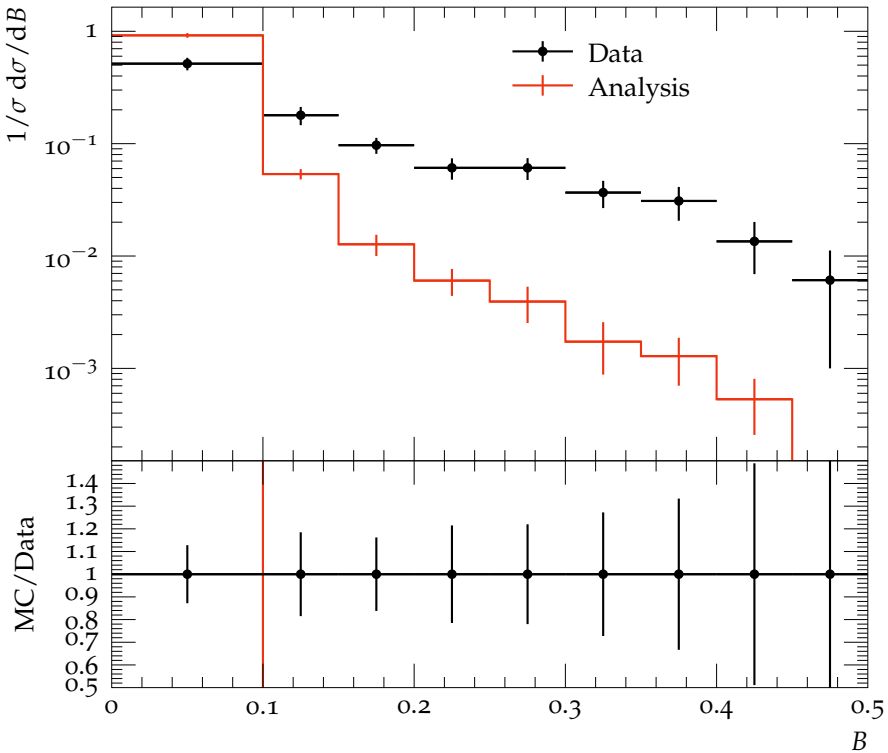
B distribution for \langle Q \rangle \leq 81\text{GeV}
