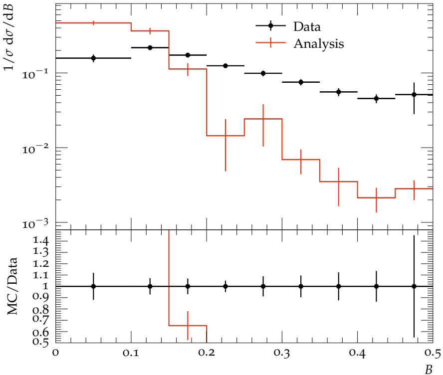
B distribution for \langle Q \rangle \leq 37\text{GeV}
