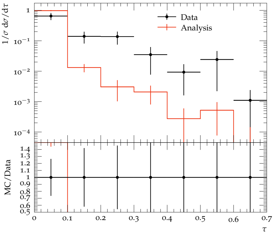
\tau distribution for \langle Q \rangle = 116\text{GeV}
