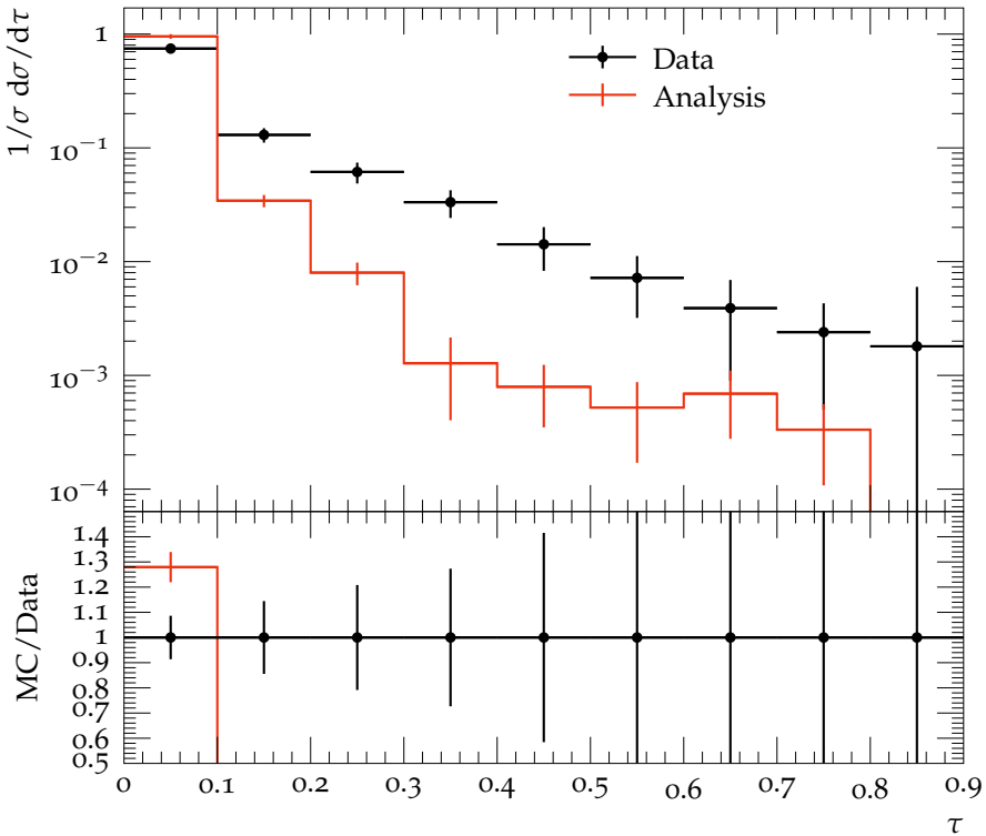
\tau distribution for \langle Q \rangle = 81\text{GeV}
