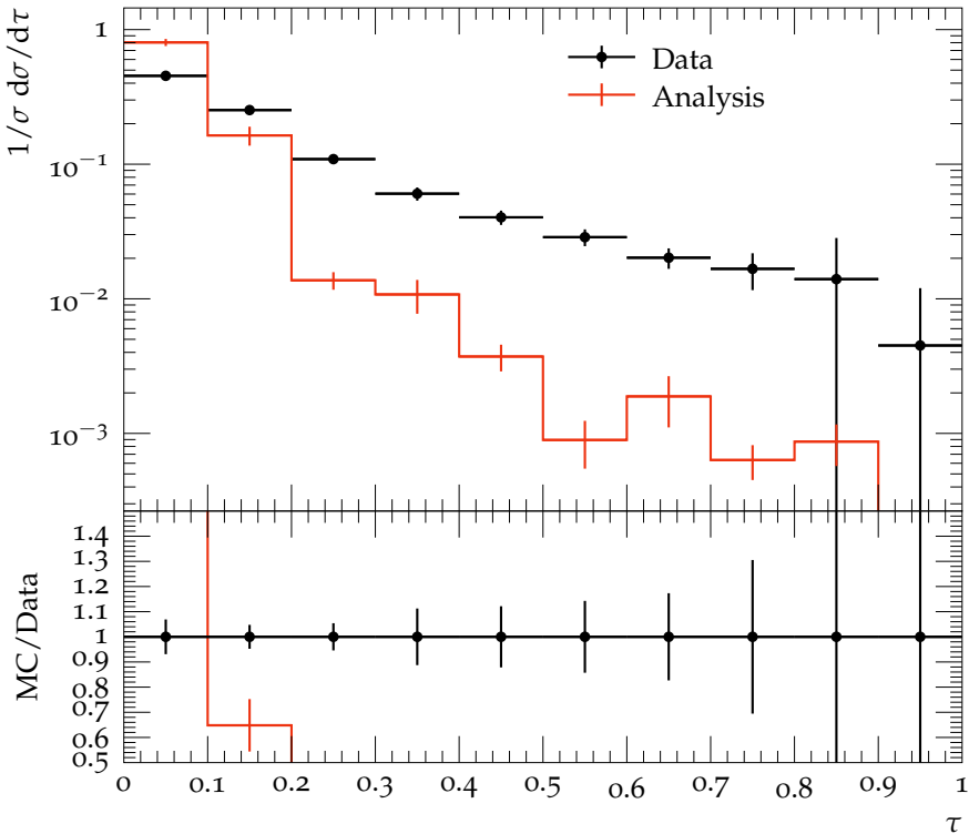
\tau distribution for \langle Q \rangle \leq 37\text{GeV}
