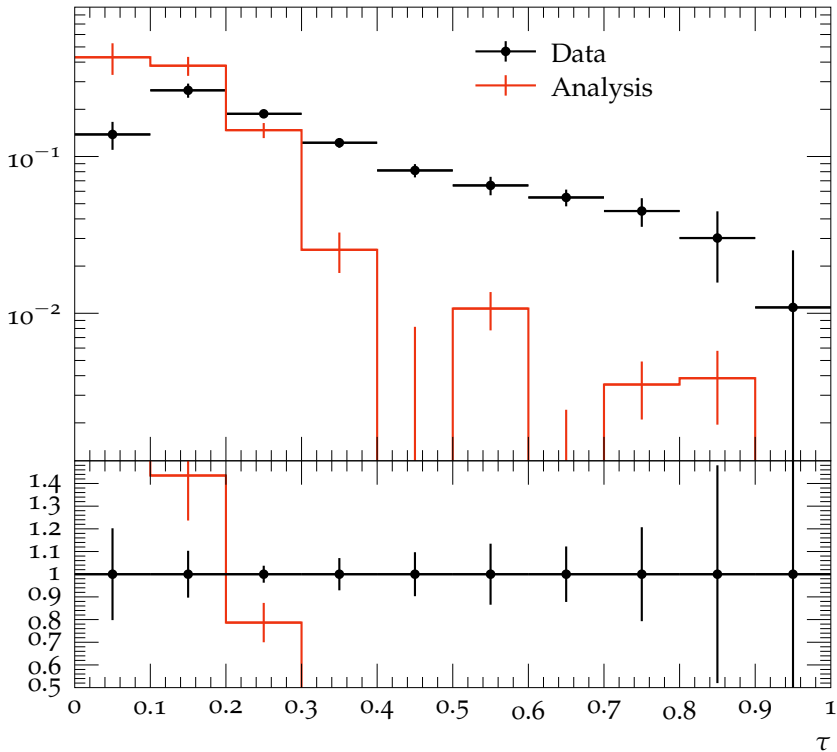
\tau distribution for \langle Q \rangle = 15\text{GeV}
