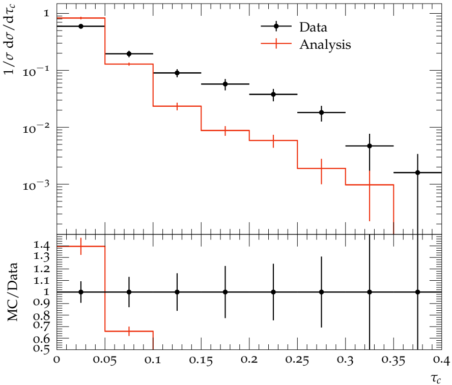
\tau_c distribution for \langle Q \rangle = 81\text{GeV}
