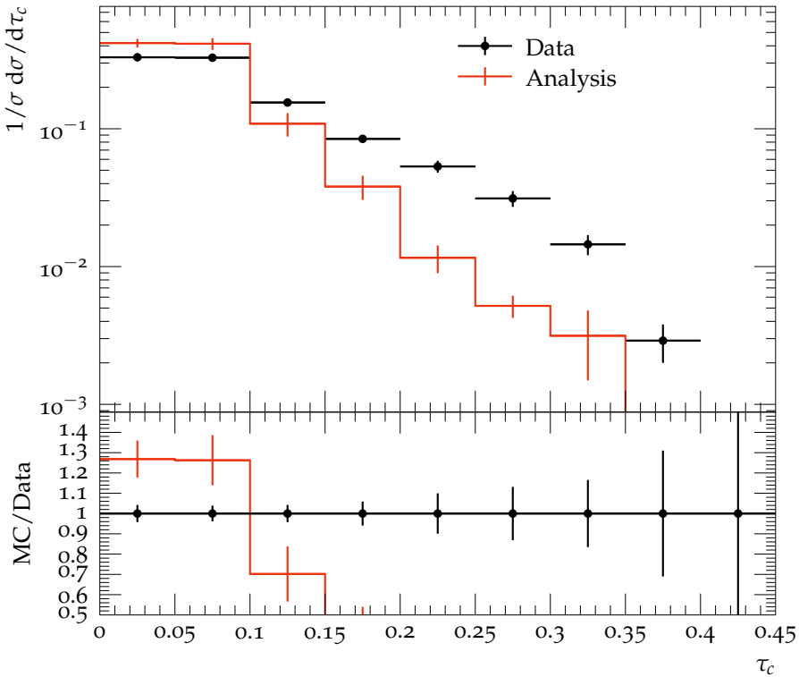
\tau_c distribution for \langle Q \rangle \geq 37\text{GeV}
