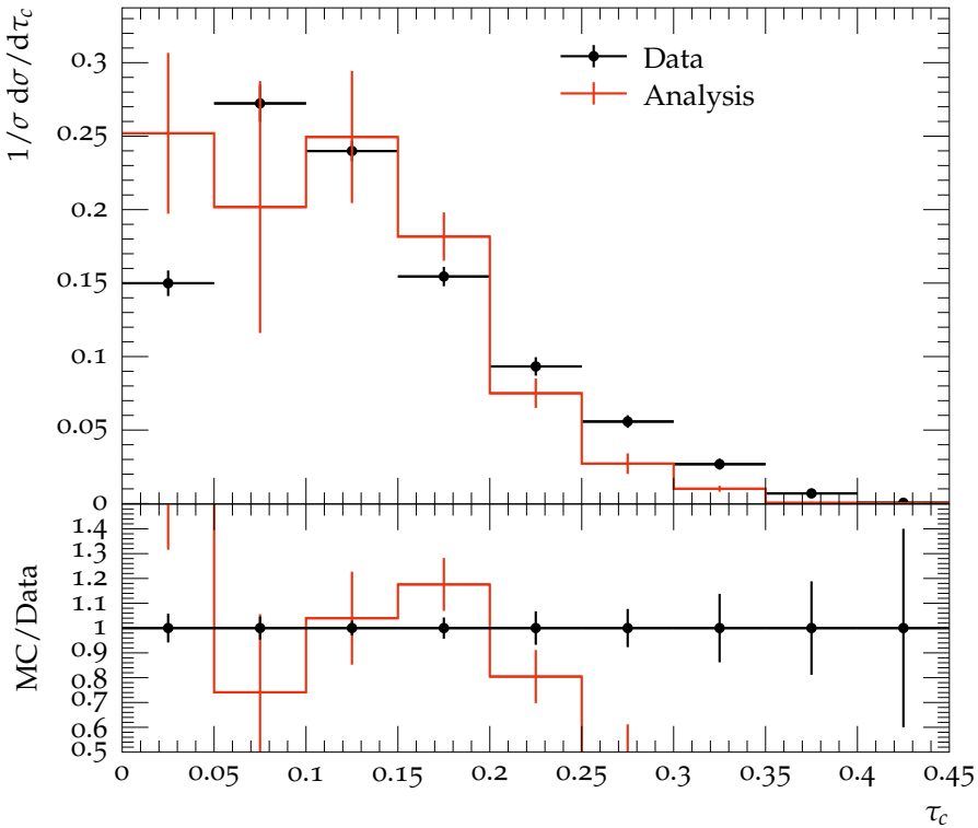
\tau_c distribution for \langle Q \rangle = 15\text{GeV}
