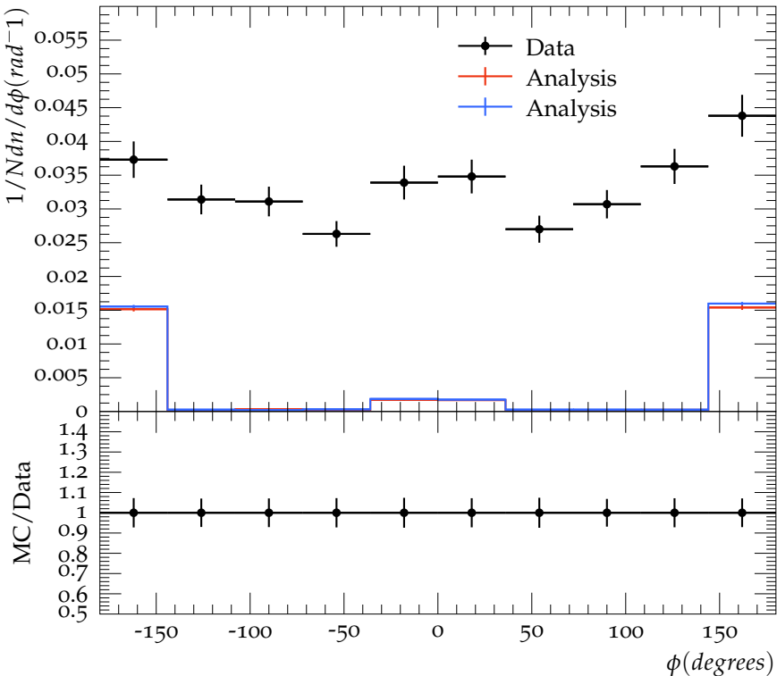
Differential \phi distribution for p_T = 1.5 GeV
