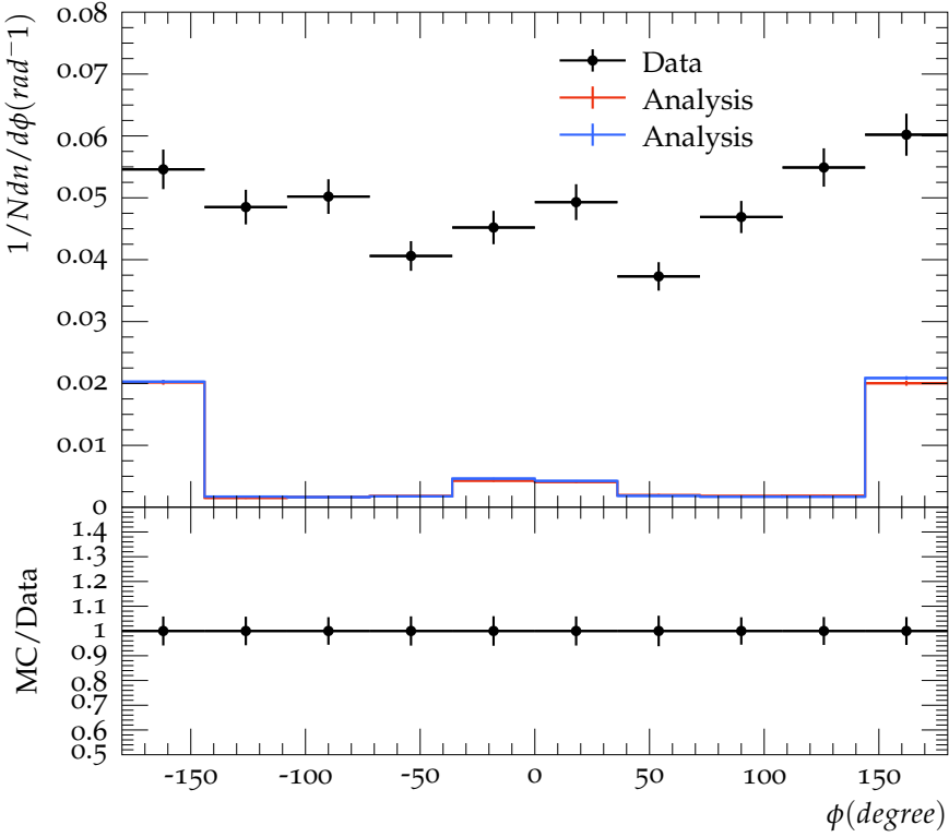
Differential \phi distribution for p_T = 1 GeV
