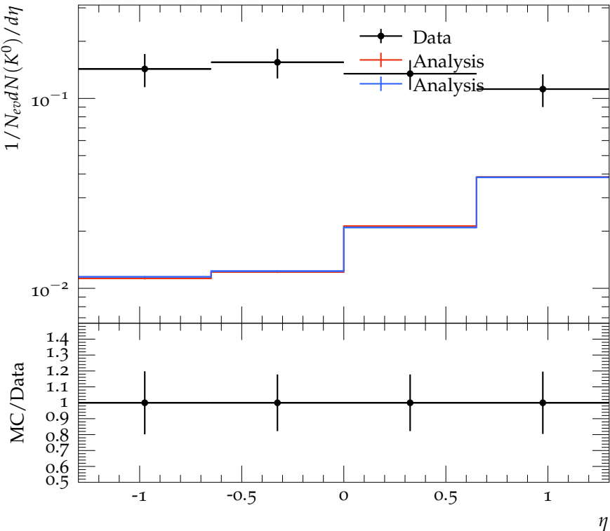
Differential K^0 multiplicity in NRG events as a function
