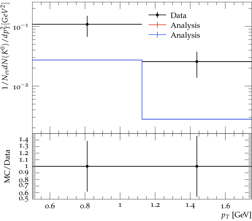
Differential K^0 multiplicity in LRG events as a function
