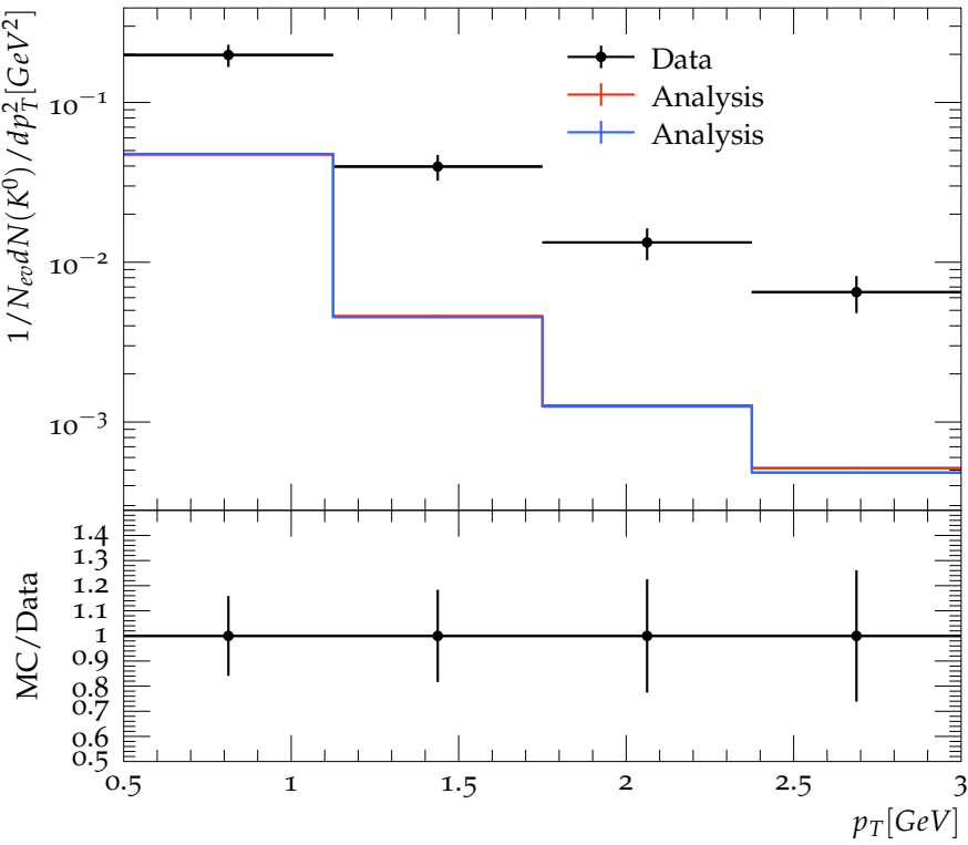
Differential K^0 multiplicity in NRG events as a function of p_T
