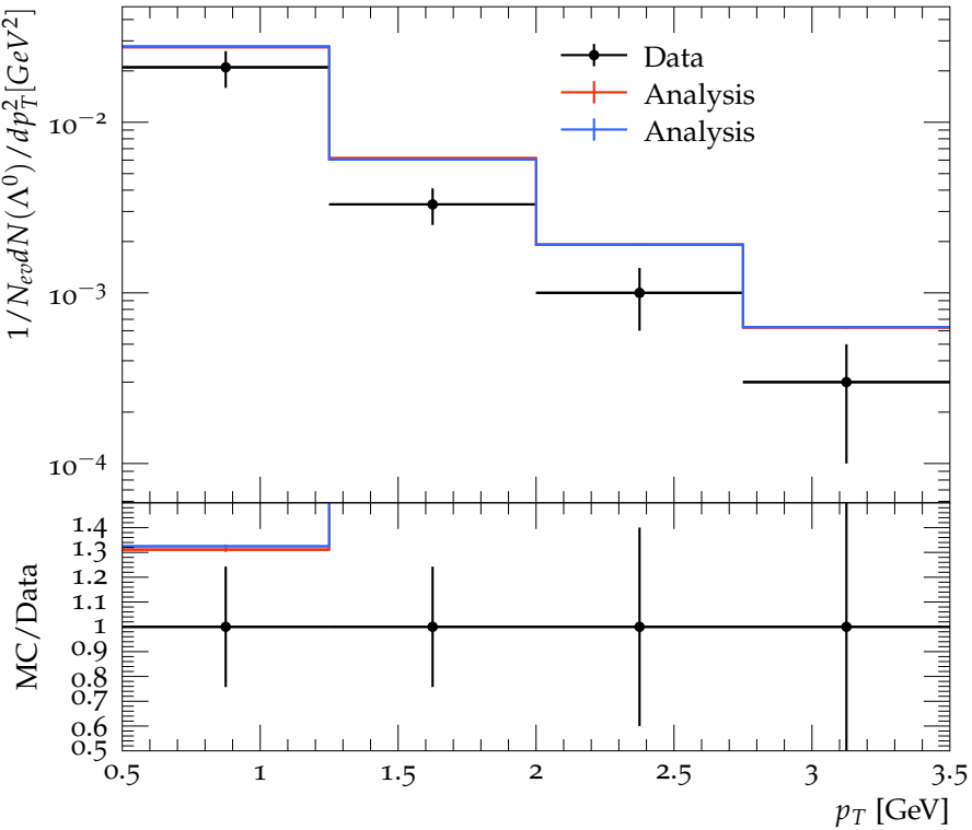
Differential multiplicity of \Lambda vs. p_T
