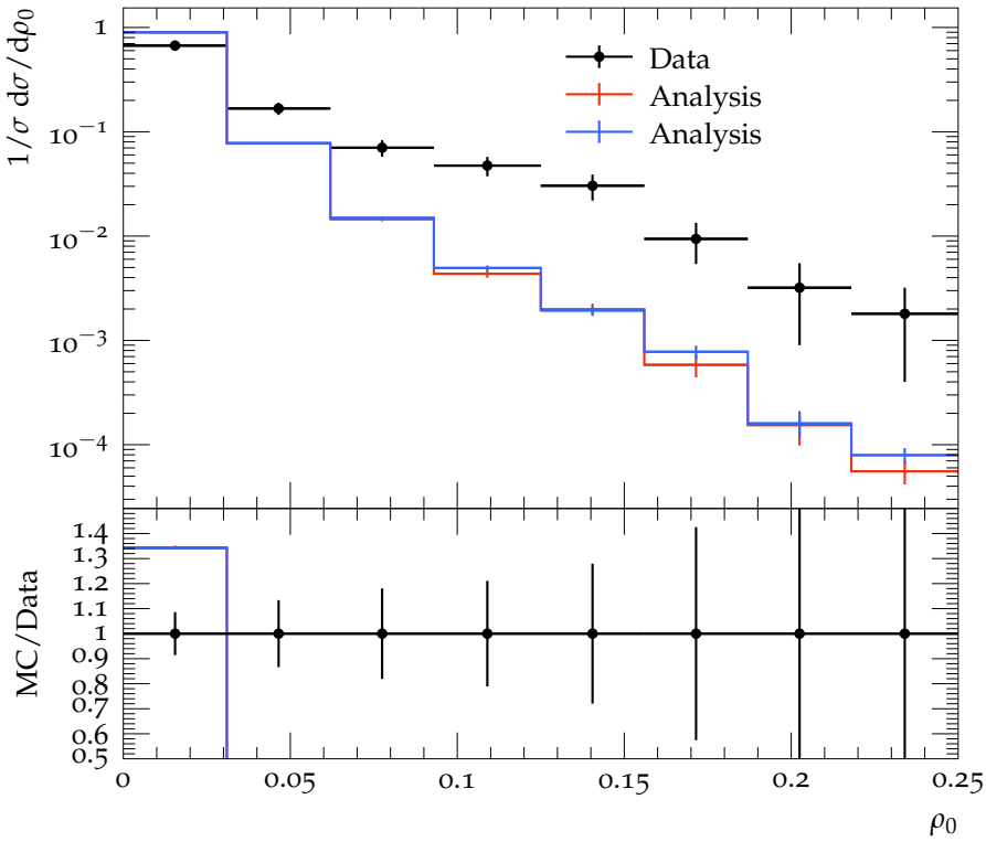
\rho_0 distribution for \langle Q \rangle = 81\text{GeV}
