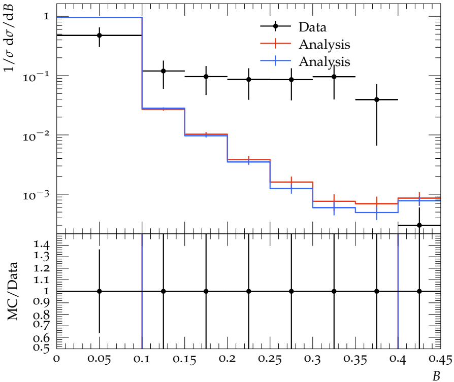
B distribution for \langle Q \rangle \leq 116\text{GeV}
