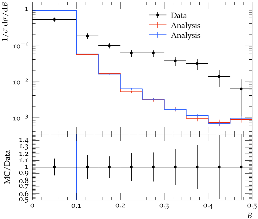
B distribution for \langle Q \rangle = 81\text{GeV}
