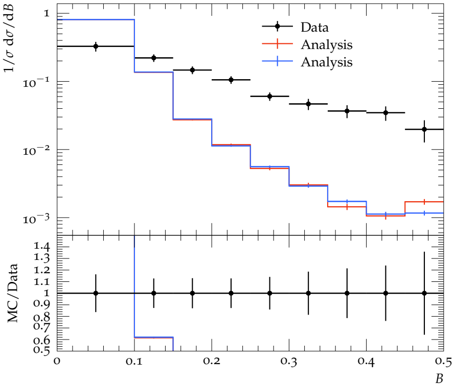
B distribution for \langle Q \rangle = 58\text{GeV}
