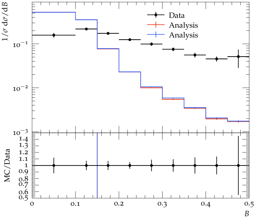
B distribution for \langle Q \rangle = 37\text{GeV}
