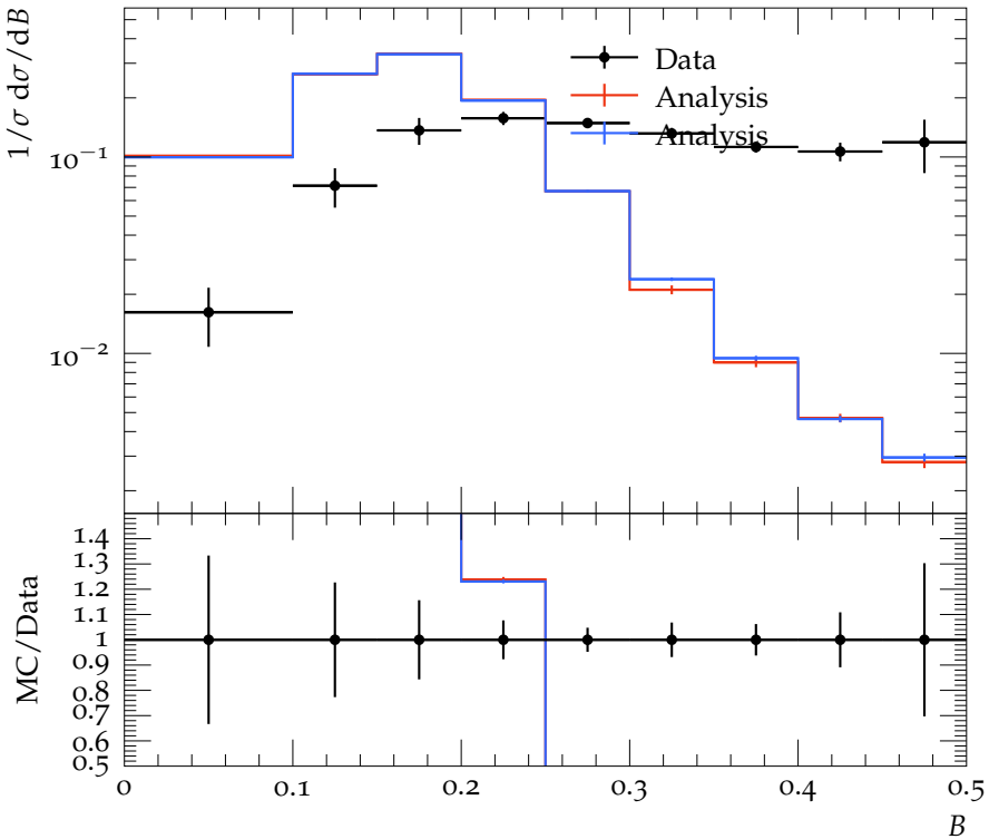
B distribution for \langle Q \rangle \leq 15\text{GeV}
