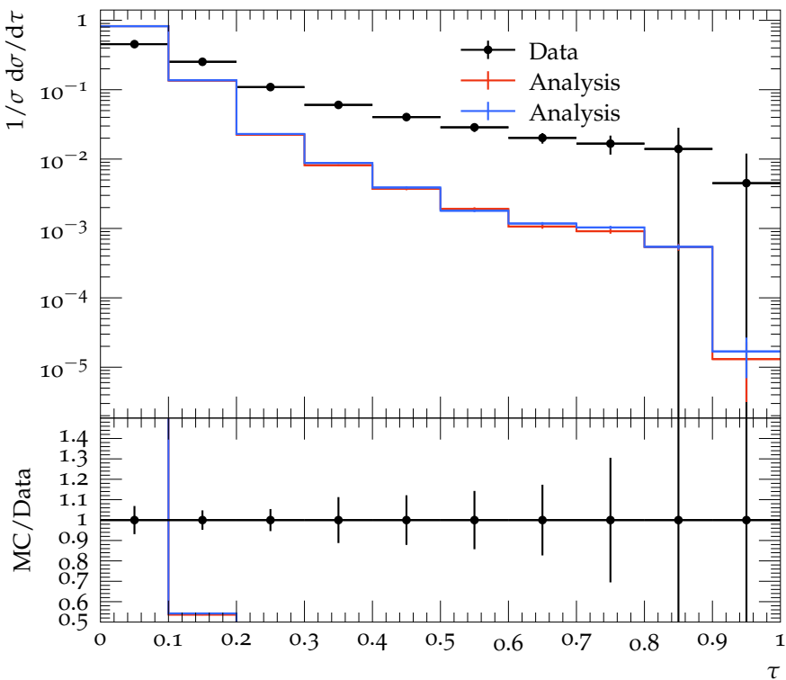
\tau distribution for \langle Q \rangle = 37\text{GeV}
