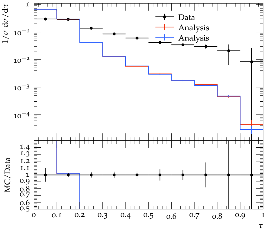
\tau distribution for \langle Q \rangle = 24\text{GeV}
