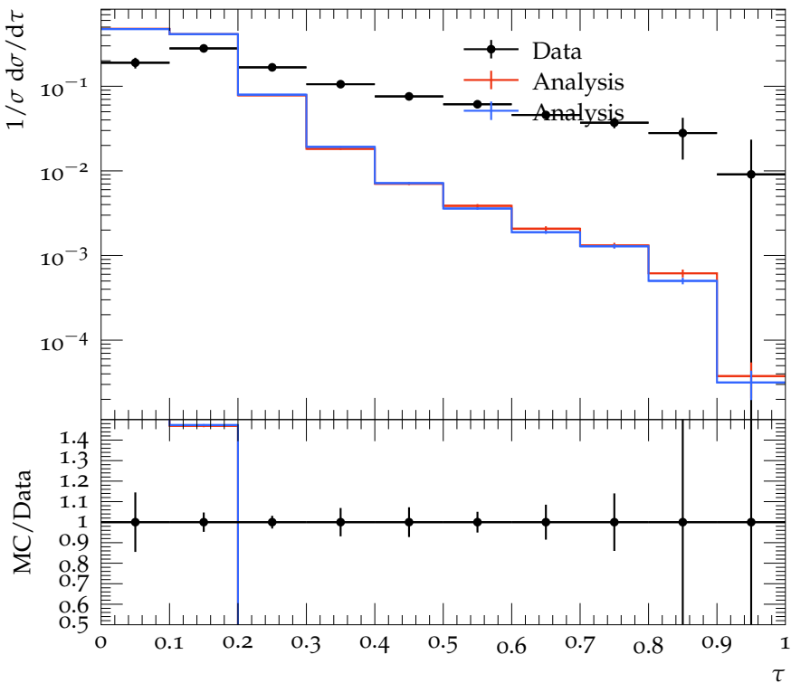
\tau distribution for \langle Q \rangle = 18\text{GeV}
