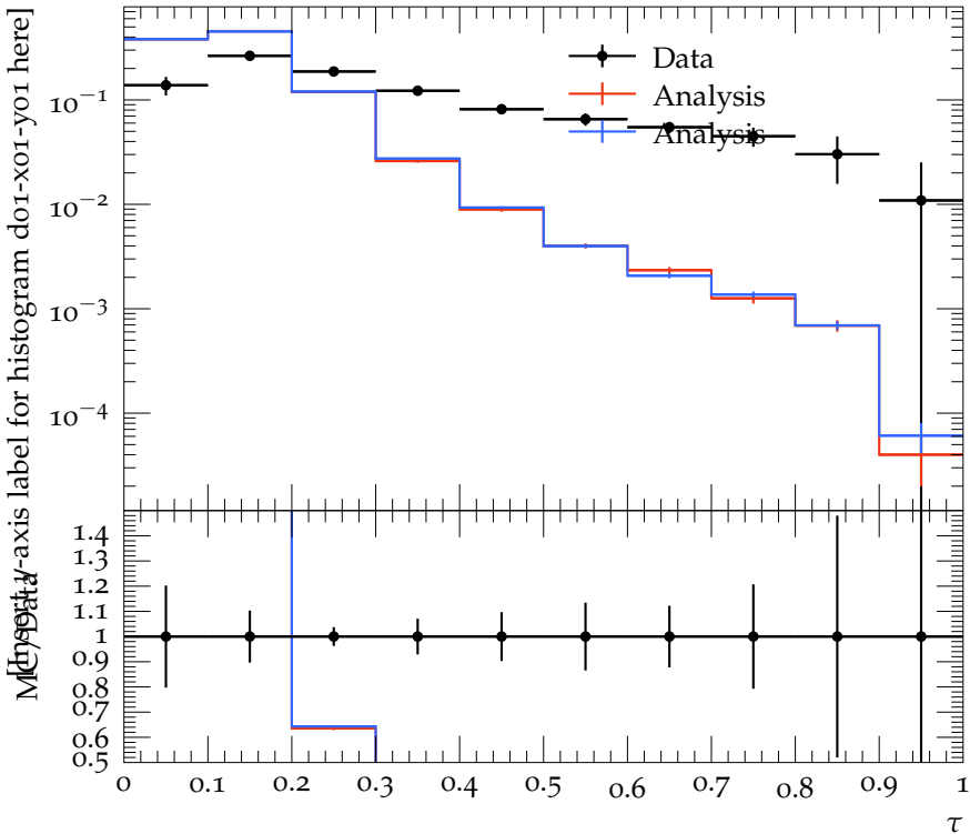
\tau distribution for \langle Q \rangle = 15\text{GeV}
