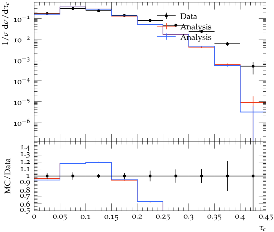
\tau_c distribution for \langle Q \rangle = 18\text{GeV}
