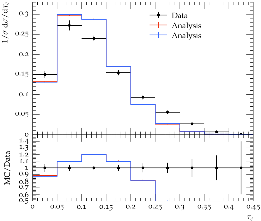
\tau_c distribution for \langle Q \rangle \leq 15\text{GeV}
