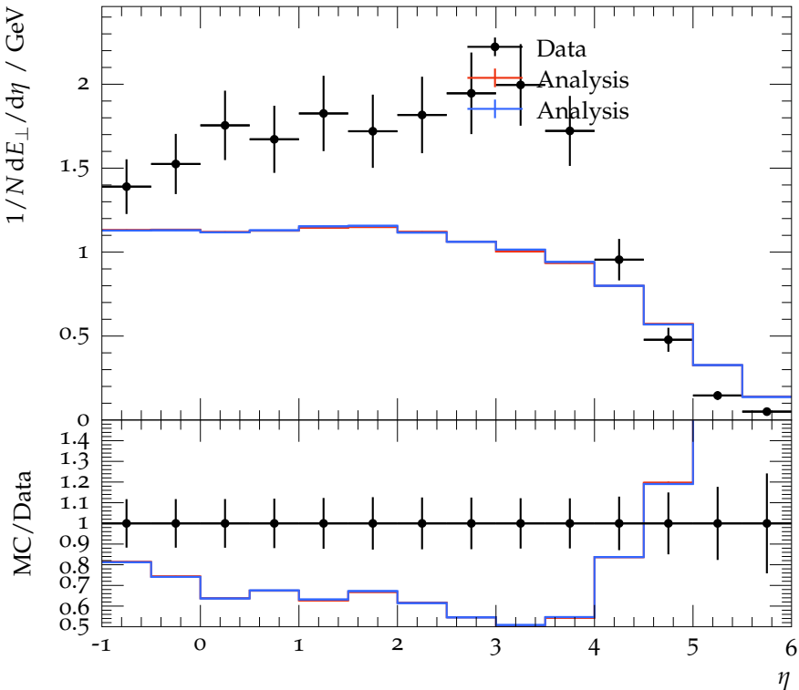
Transverse energy flow for \langle Q^2 \rangle = 5 - 10 \text{ GeV}^2
