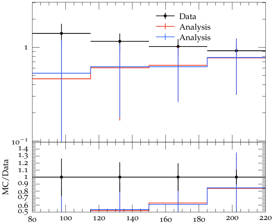
R_3 vs W , 4 < \eta < 5
