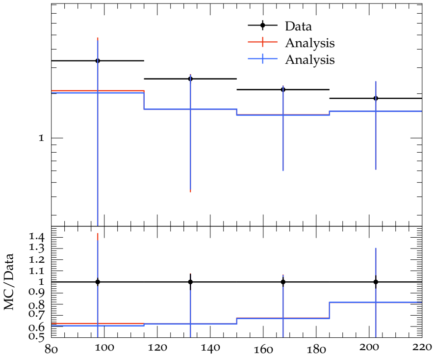
C_2 vs W , 4 < \eta < 5
