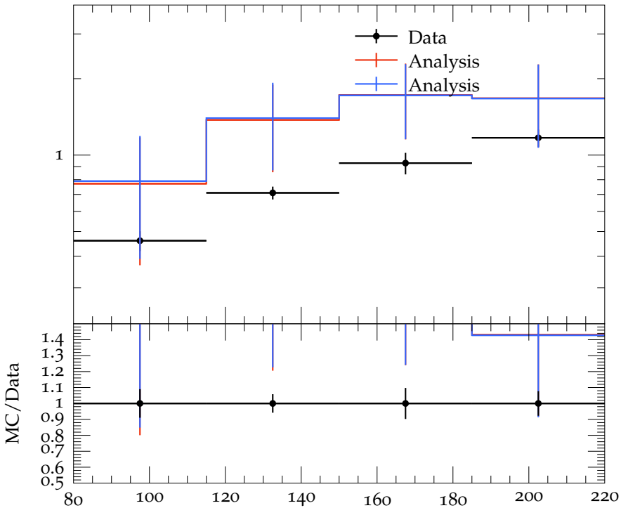
Mean multiplicity vs W , 4 < \eta < 5
