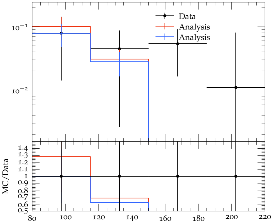
K_3 vs W , 3 < \eta < 4
