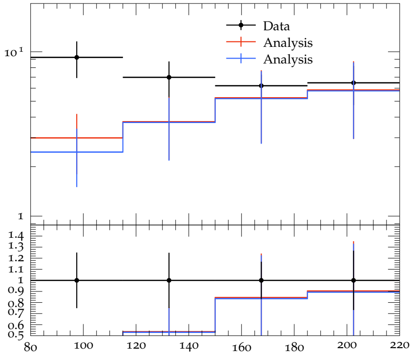
C_4 vs W , 3 < \eta < 4
