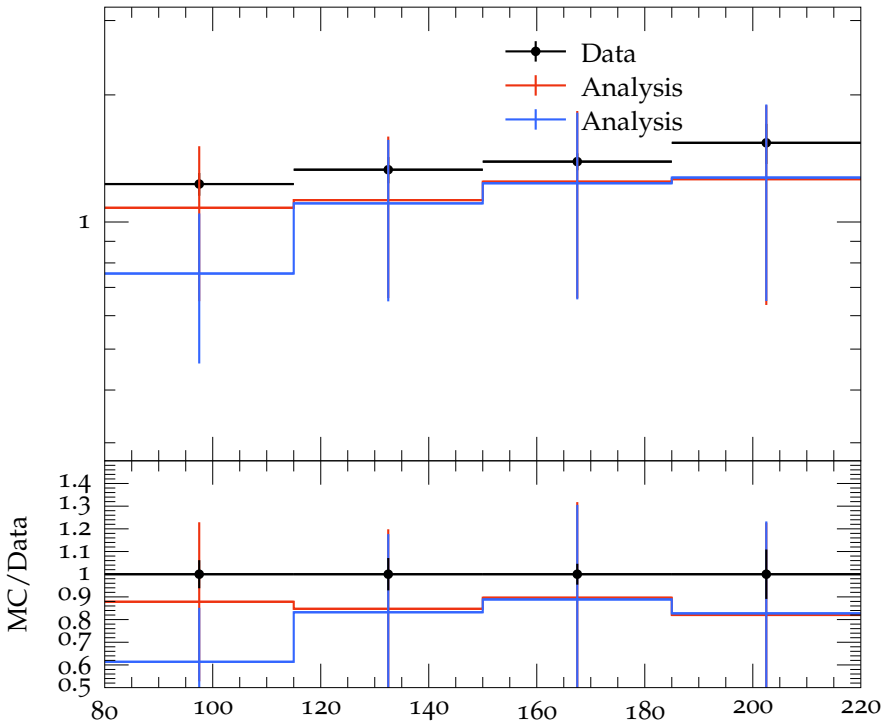
D_3 vs W , 3 < \eta < 4
