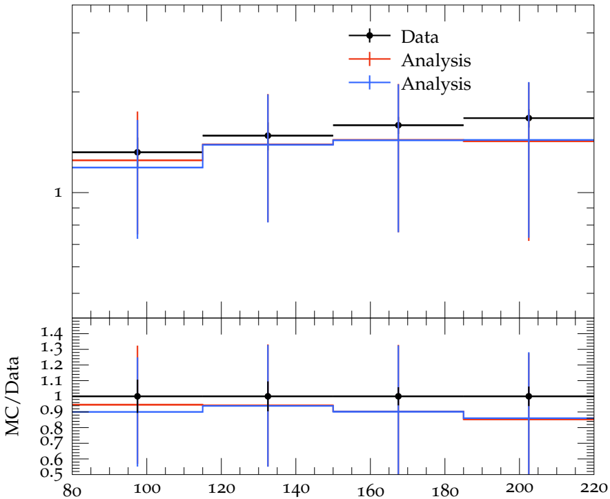
D_2 vs W , 3 < \eta < 4
