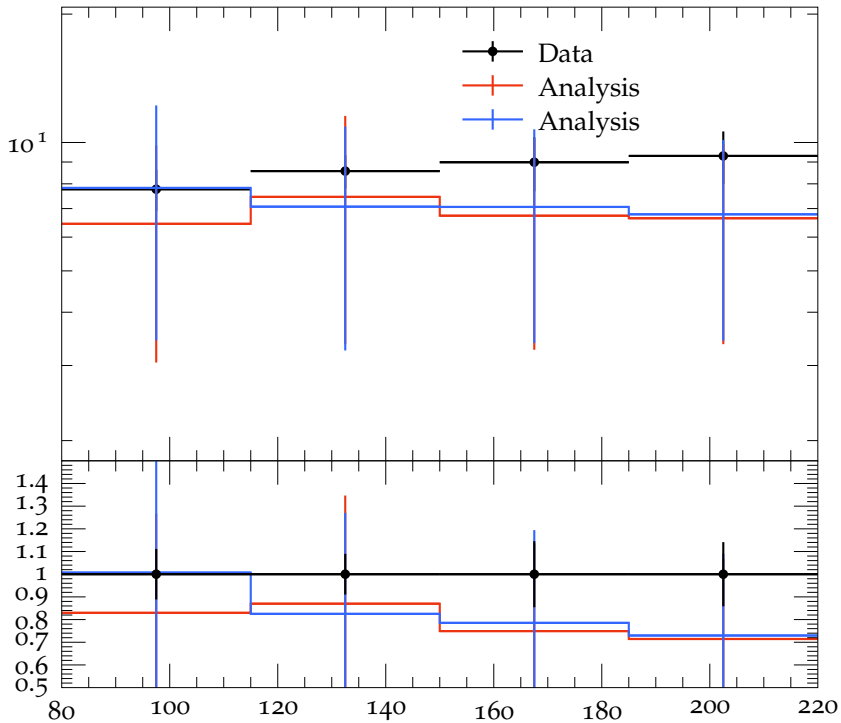
C_4 vs W , 2 < \eta < 3
